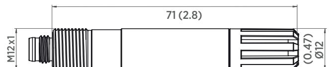
Dimensions in mm (inches)
