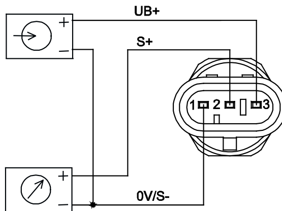
AMP Superseal
