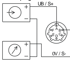
MIL-plug PT 02 E-10 6P
