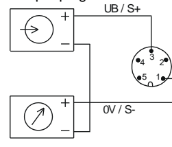
5-pin plug
