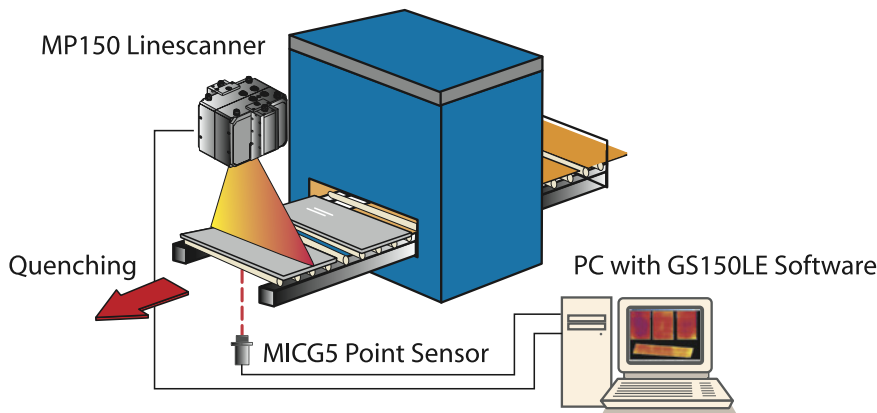
Basic set-up of the GS150LE System
